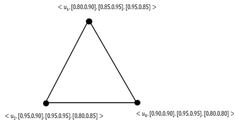
Figure 10. Interval – valued Fermatean Neutrosophic Graph G_2
