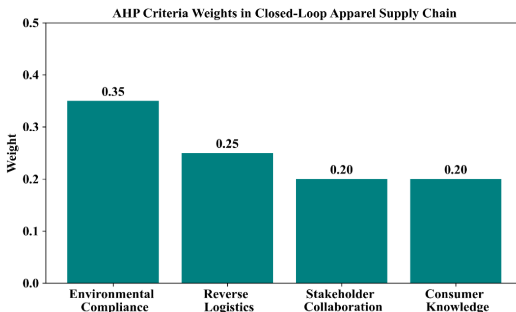
Fig.2: AHP Weights
