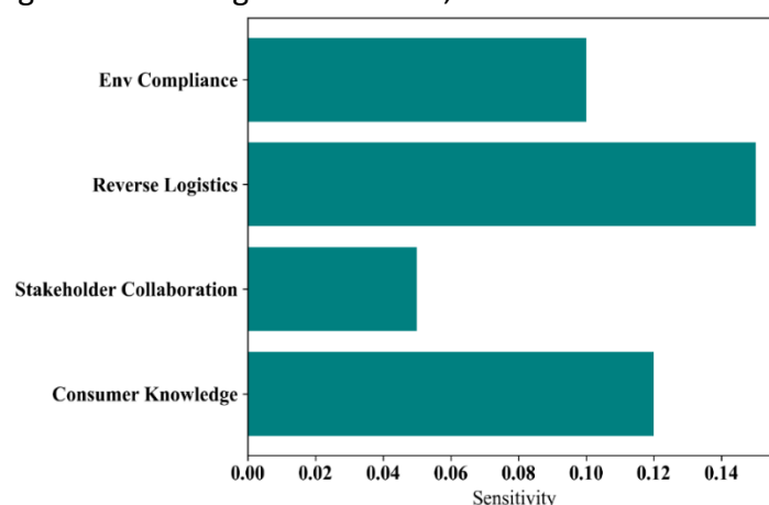
Fig.10: Sensitivity Analysis
