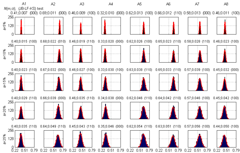
Figure 1. Histogram of the relative closeness to the ideal solution depending on the relative error in the data ( \delta, \% ). (1000 Simulation of DM Matrix; m, \sigma - parameters of normal distribution)
