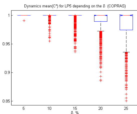
Figure 3. Dynamics mean ( C_5^* ) depending on \delta . (A 5 , COPRAS, 1000 Simulation of DM Matrix).
