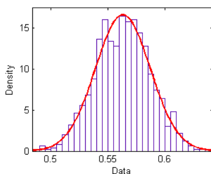
Figure 2. Fit distributions to C_5^* (LC5, COPRAS, \delta=20\% , 1000 Simulation of DM Matrix)
