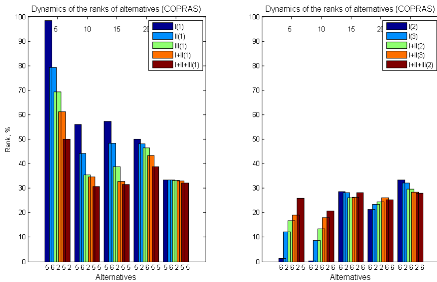
Figure 4. Distribution of the point of realizations of effective alternatives in% to the total number of N experiments having ranks I, II, III, and the sums I+II, I+II+III ranks (LC5, COPRAS, 1024 Simulation of DM Matrix, \delta = 5-25\% )
