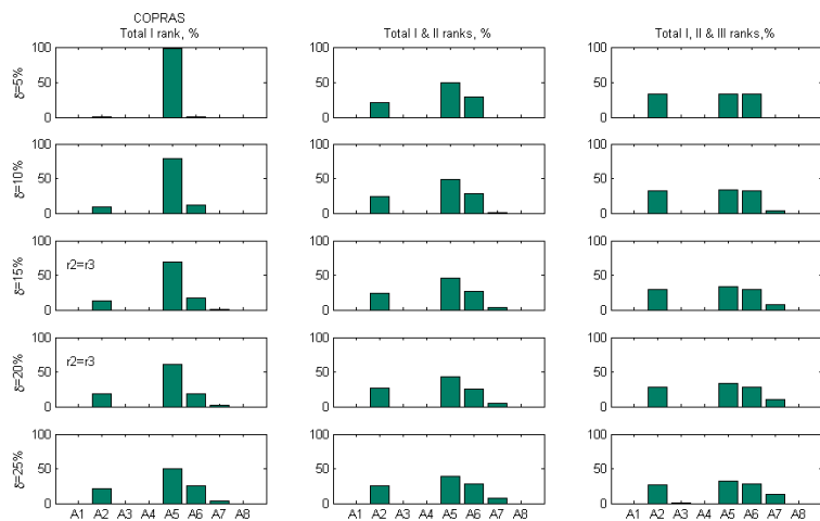
Figure 5. Distribution of the point of realizations of effective alternatives in% to the total number of N experiments having ranks I(1) and the sums I + II(1), I + II + III(1) ranks. (COPRAS, 1024 Simulation of DM Matrix, \delta = 5\text{--}25\% )
